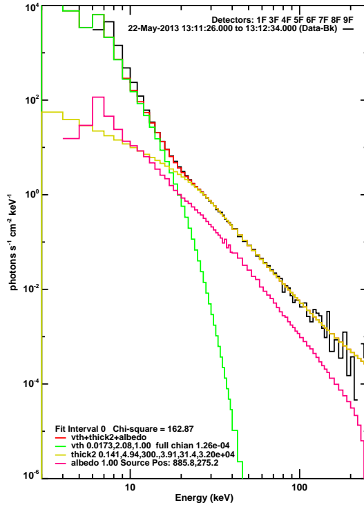
Figure 4. X-ray spectrum fitted with a power-law, thermal distribution and correcting for albedo.
